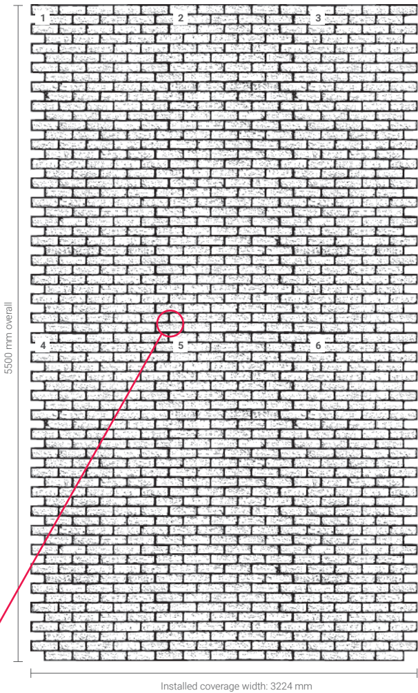
SIX PANEL LAYOUT Pattern repeats horizontal & vertical
