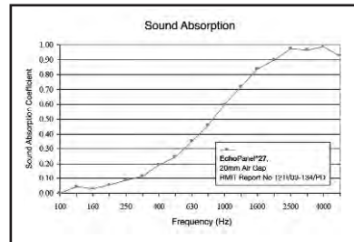
Graph: Sound Absorption Coefficients of Woven Image EchoPanel®27 tested with a 20mm air gap
